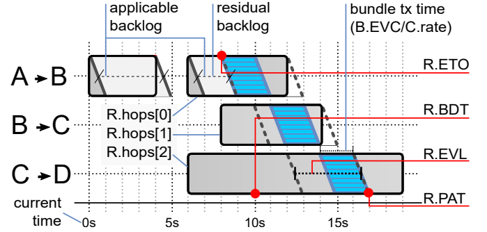
Figure 12. Illustration of parameters computed in Alg. 5. Applicable backlog is the total volume in queue at current time, while residual backlog is the part of that volume affecting the current route. Bundle transmission time is the time needed to transmit the whole bundle on the channel. These parameters are needed to evaluate the route considering bundle size and queue status.
