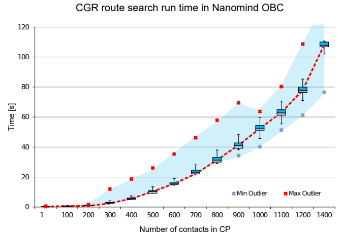
Figure 13. CGR route search (Alg. 1) run time in GomSpace's Nanomid A712C on-board computer with Free RTOS clocking at 10 MHz (implemented in C language). The contact plan corresponds to a Walker constellation of 12 satellites, 10 ground stations, and 100 ground spots for a duration of 24 hrs. [87]. Results are averaged among traffic from all ground sites to a mission control center reachable through any of the ground stations. The number of contacts considered ranges from 1 to 1400, at which point the OBC's 2MB of static RAM are exhausted. Courtesy of the Argentinian Space Agency (CONAE, Unidad de Formación Superior).
